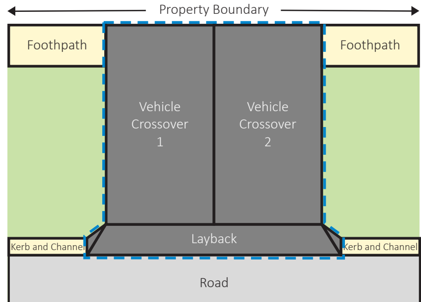
Figure 4. Adjoining vehicle crossover example
