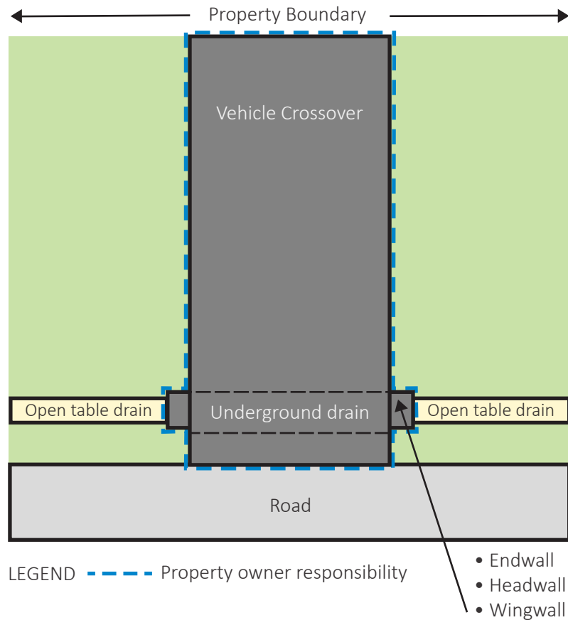
Figure 2. Rural vehicle crossover example
