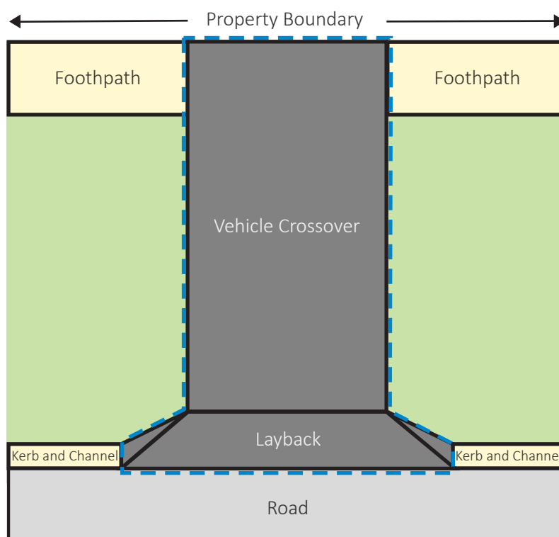
Figure 1. Urban vehicle crossover example
