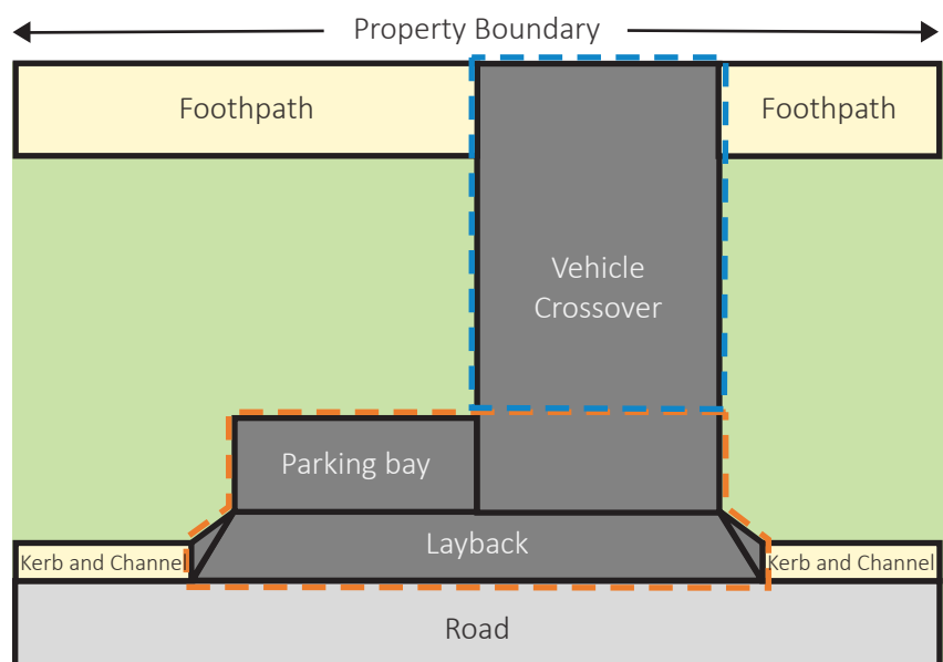
Figure 5. Adjoining parking bay/vehicle crossover example
