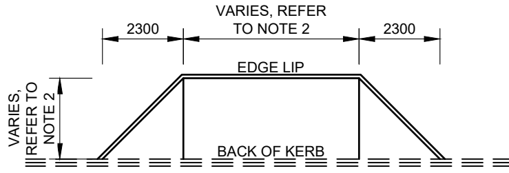
SINGLE BAY WITH TAPERED ENDS
