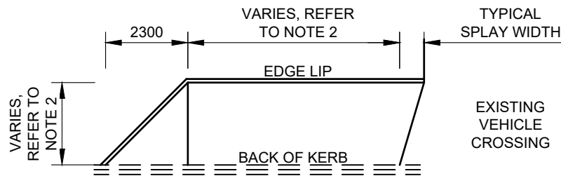
SINGLE BAY NEXT TO VEHICLE CROSSING
