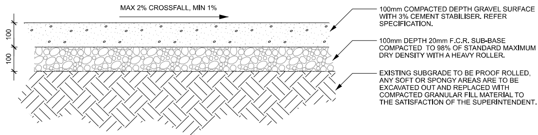
1 COMPACTED GRAVEL FOOTPATH TYPICAL DETAIL 1:10
