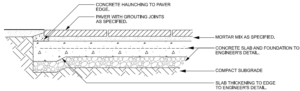
1 PAVING ON CONCRETE BASE TYPICAL DETAIL 1:10
